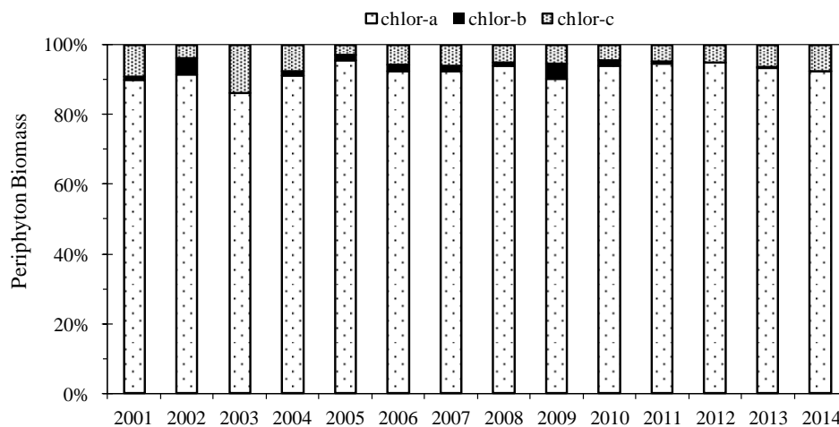
Figure 22.—Tributary Creek Site 9 mean chlorophylls a , b , and c proportions.
