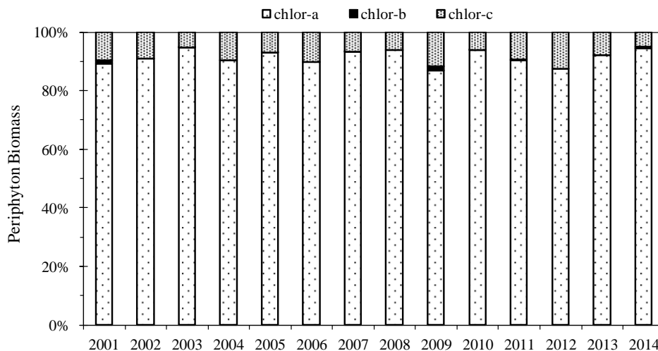
Figure 10.—Greens Creek Site 48 mean chlorophylls a , b , and c proportions.
