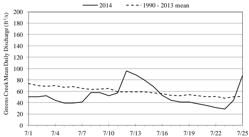
Figure 7.—Greens Creek mean daily discharge (ft 3 /s) three weeks prior to sampling in 2014, and mean daily discharges for the period 1990–2013. Source: USGS Gage 15101490 (USGS 2015).
