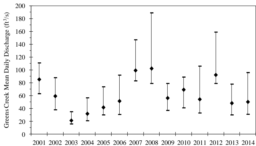
Figure 8.—Greens Creek mean daily discharges three weeks prior to sampling. Note: Median (♦), minimum, and maximum mean daily discharges ((ft 3 /s) presented). Source: USGS Gage 15101490 (USGS 2015).
