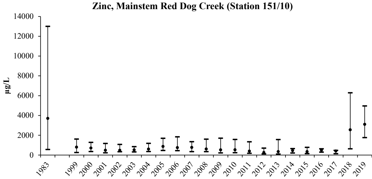
Figure 7. Median, maximum, and minimum zinc concentrations at Station 151/10.
