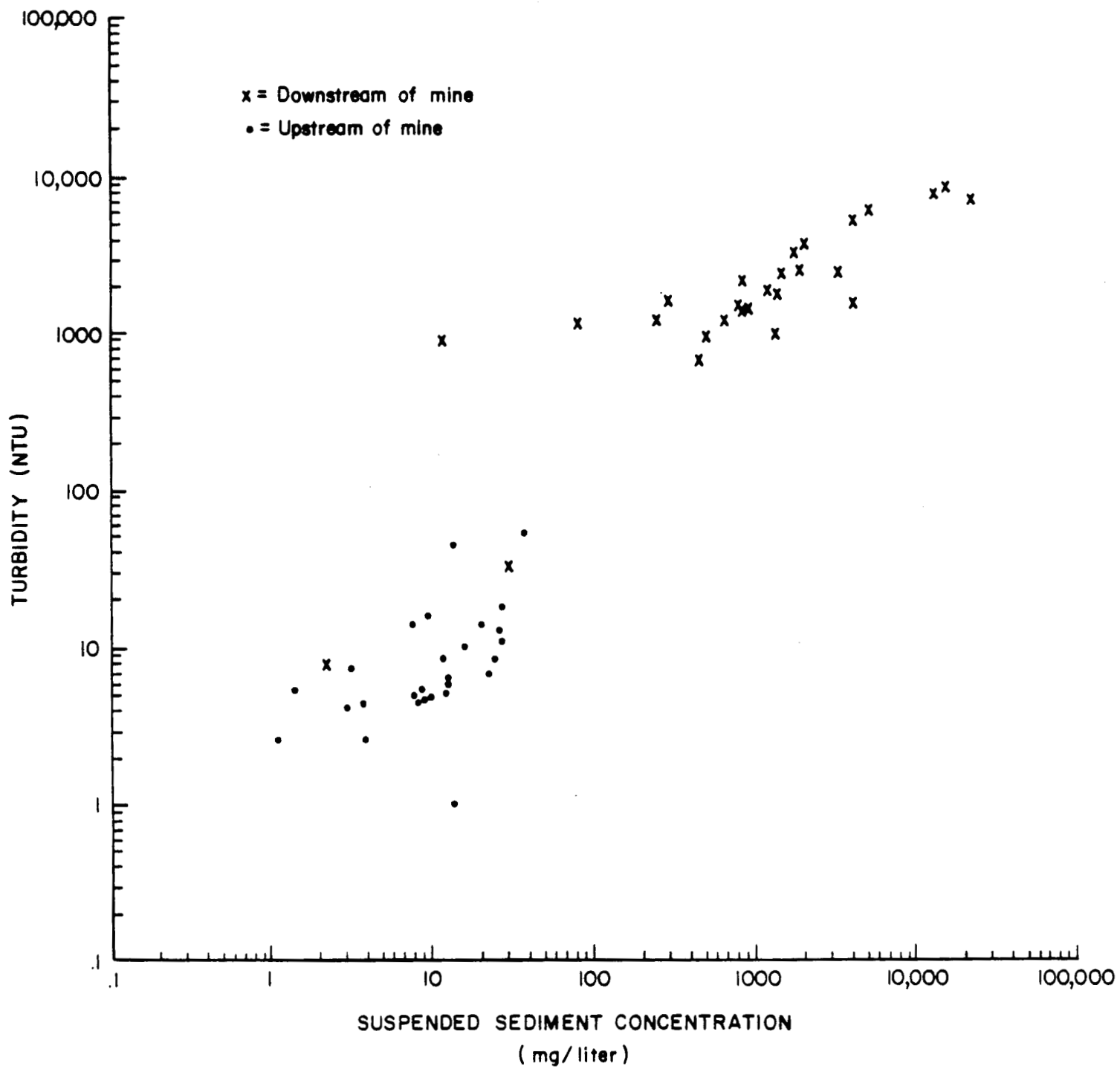
Figure 11. Plot of turbidity and suspended sediment concentration for certain placer-mined streams in Alaska (plotted in this report from data presented in R&M Consultants, 1982a).
